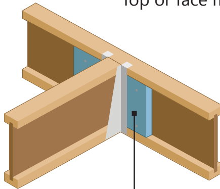
Top or face mount hanger
